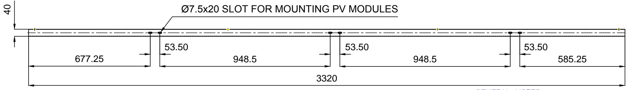
FRONT VIEW
