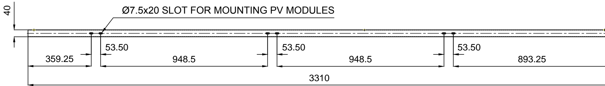
FRONT VIEW
