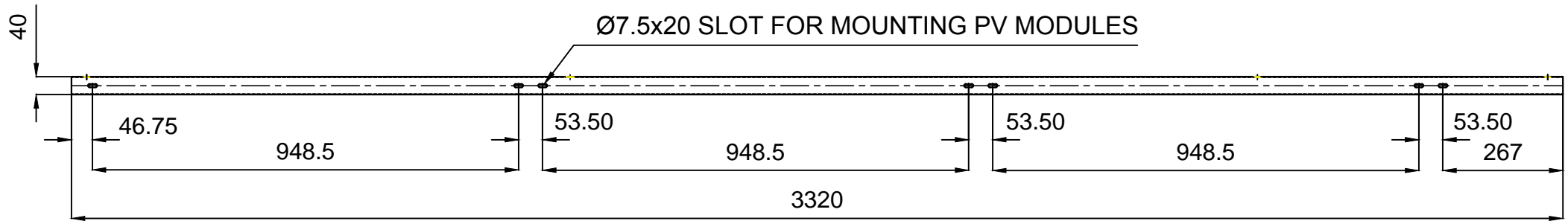
TOP VIEW
