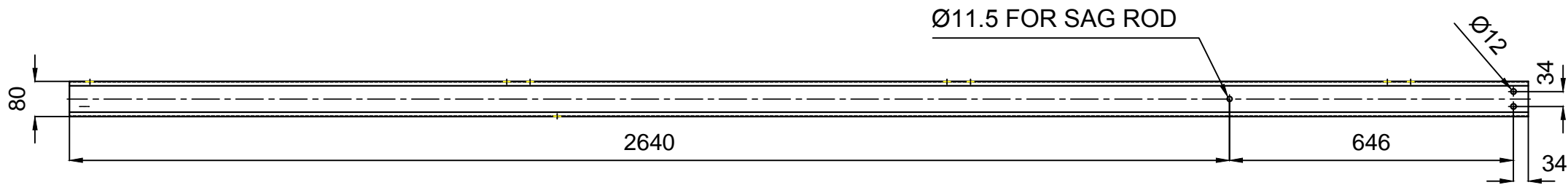
FRONT VIEW
