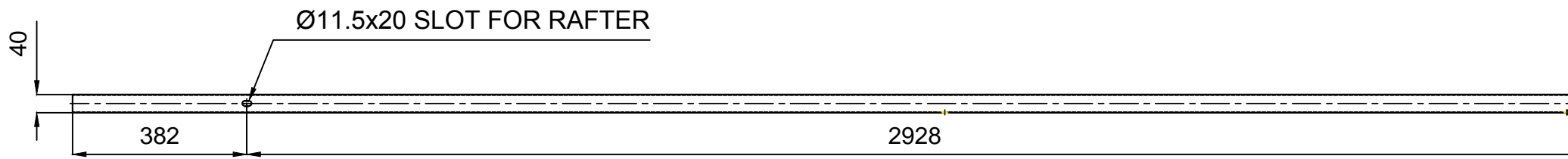
BOTTOM VIEW
