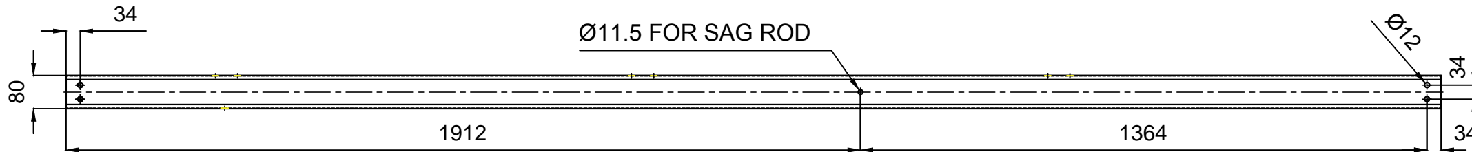
FRONT VIEW
