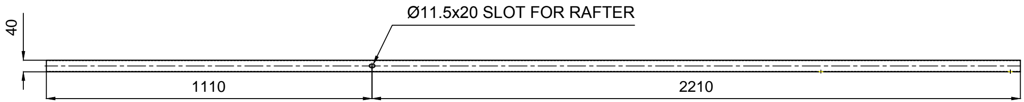
BOTTOM VIEW
