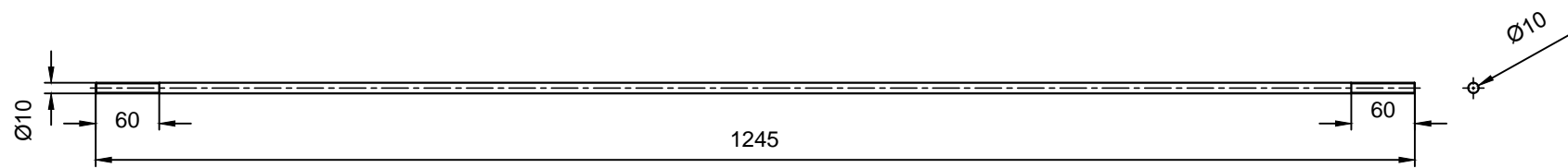
FRONT VIEW
